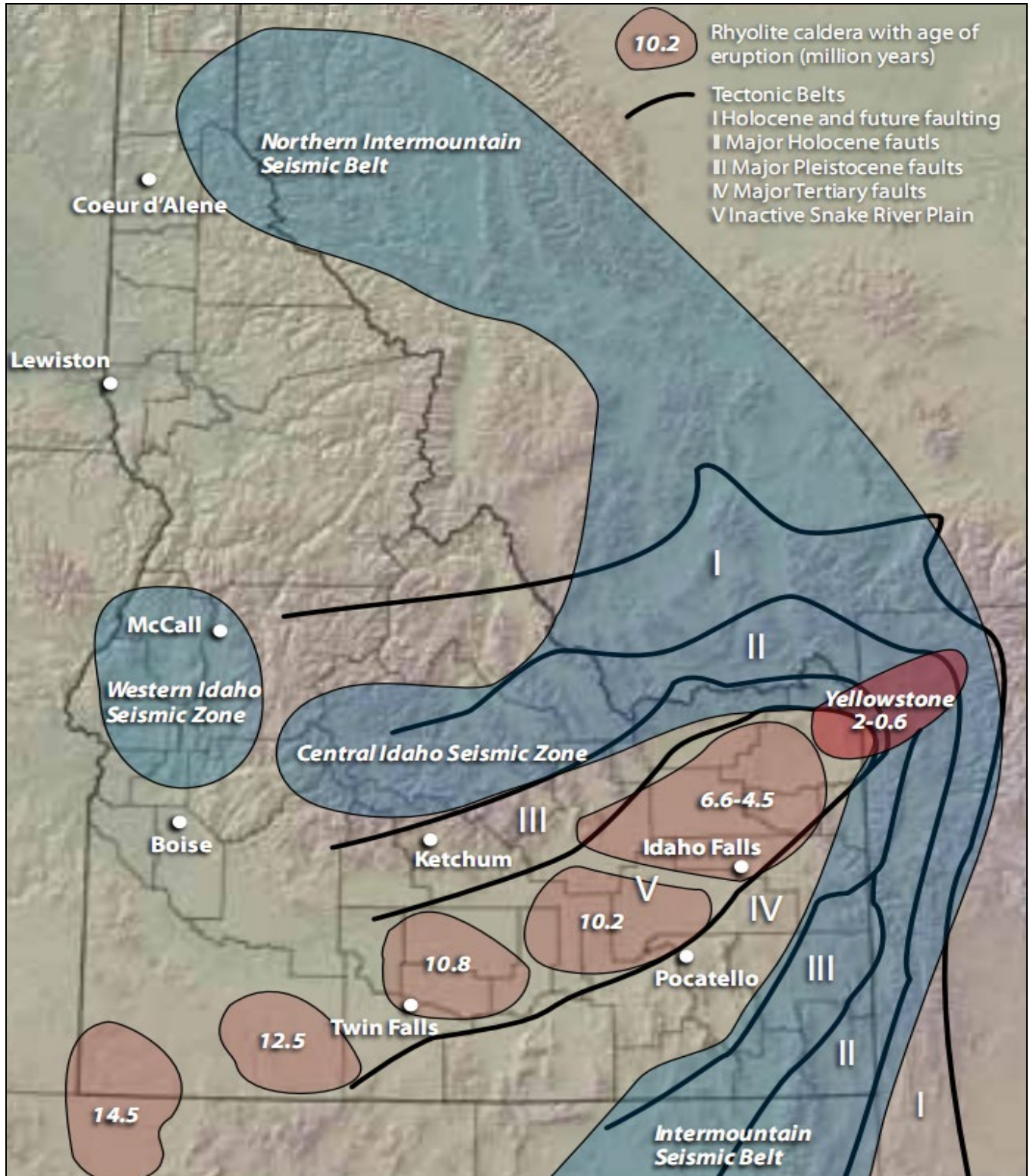
Figure 11-2. Volcanic and Tectonic Features of the Yellowstone-Snake River Plain System
