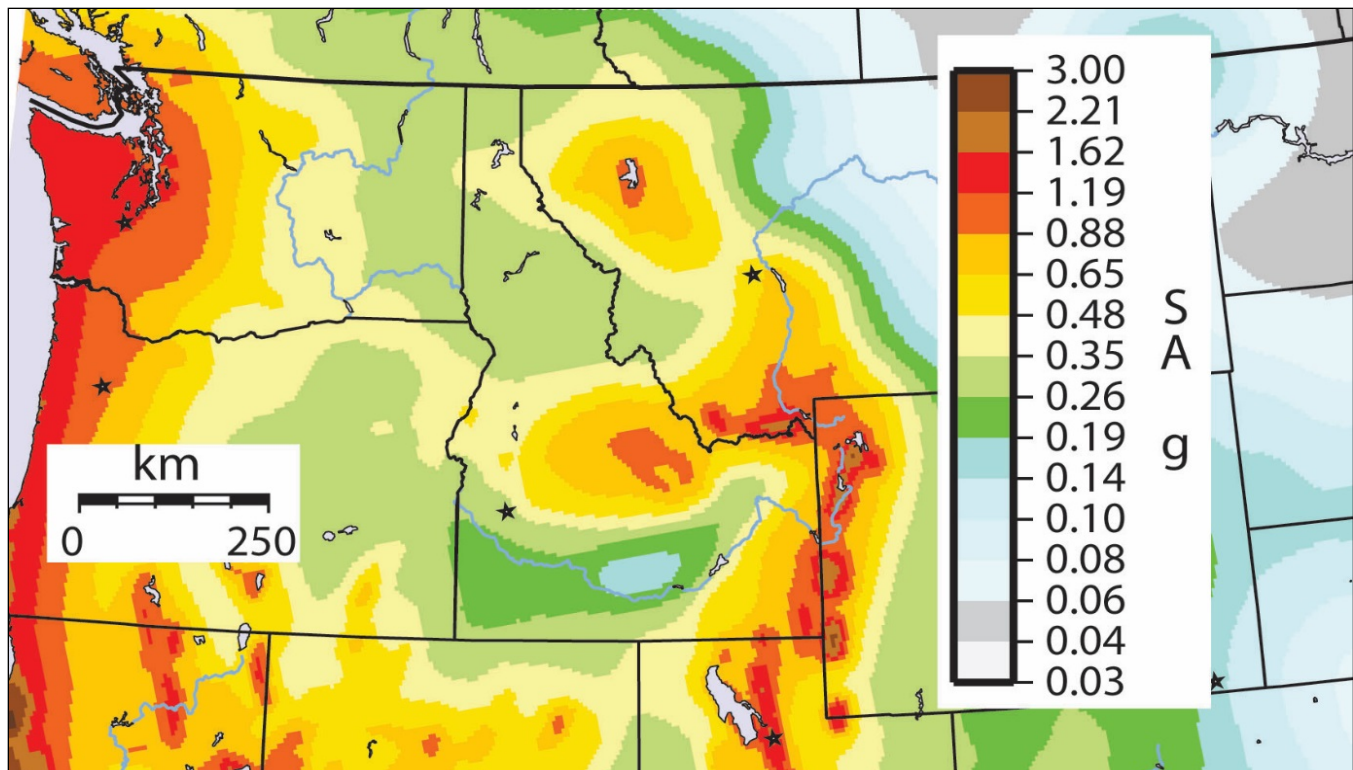
Figure 11-8. PGA with 2-Percent Probability of Exceedance in 50 Years, Northwest Region
