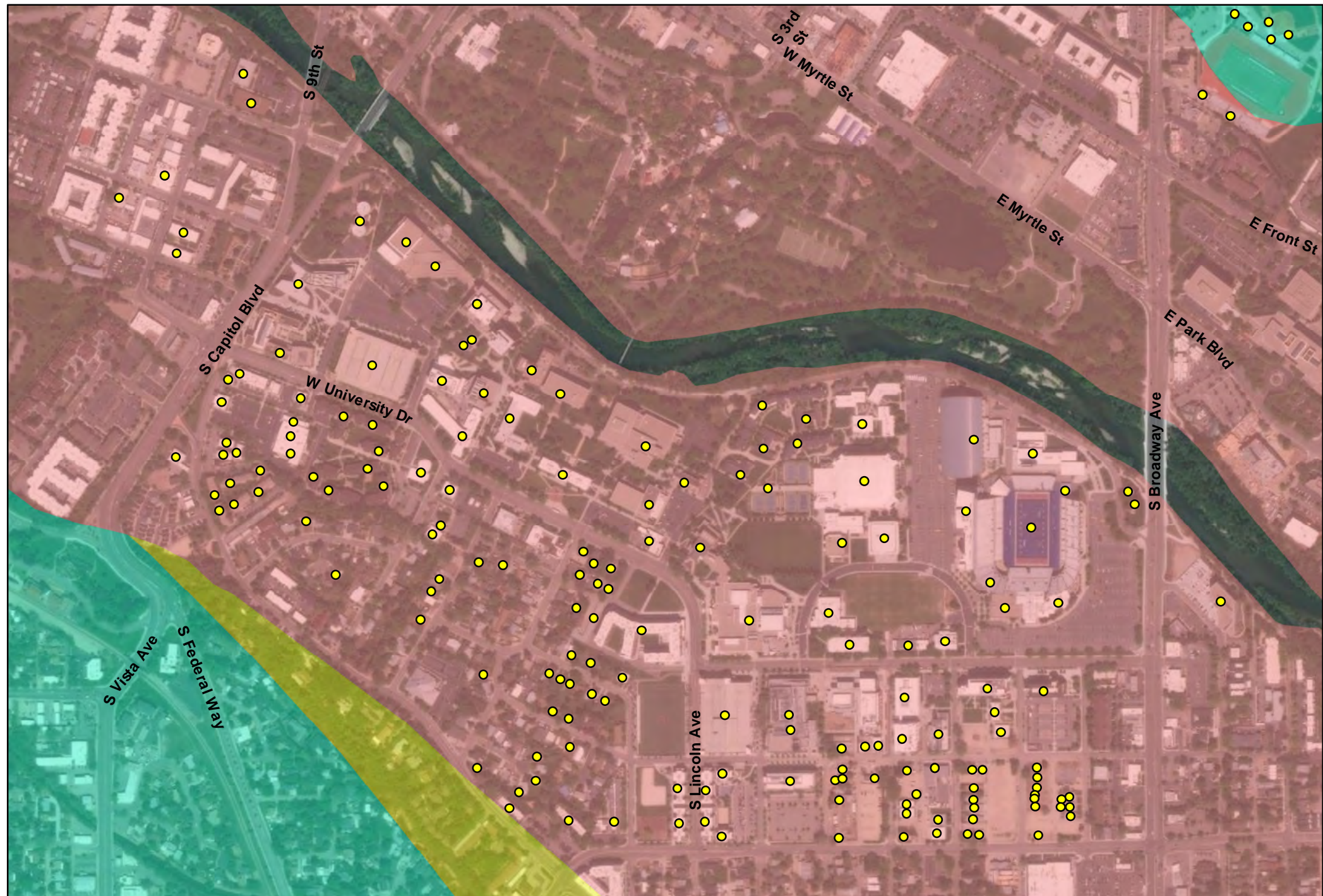
Figure 11-7a. Liquefaction Susceptibility
