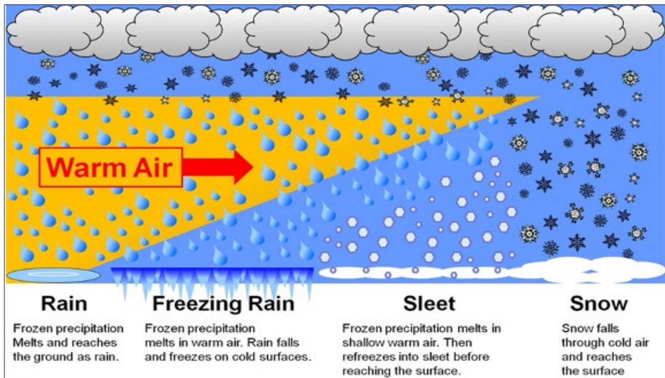
Figure 17-2. The Formation of Different Kinds of Precipitation
