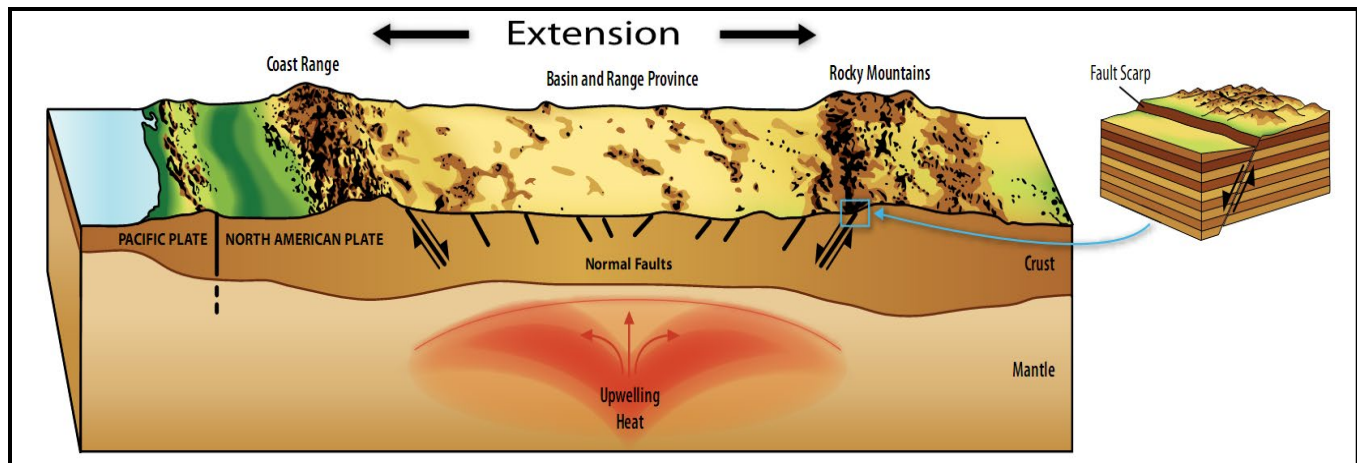
Figure 11-1. Horizontal Extension Creates Normal Faults
