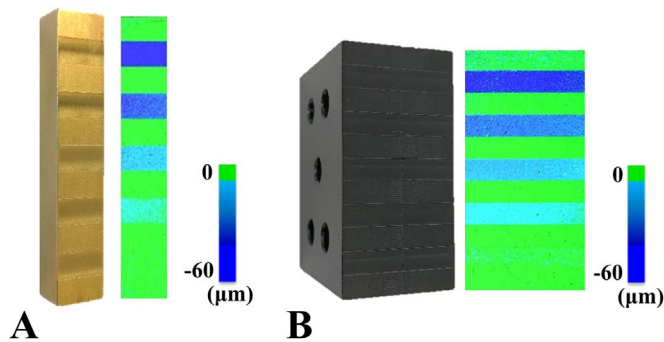
Fig. 5. Reference blocks with machined recesses were used to produce colorimetric maps of linear wear depth for A) metal and B) plastic materials.
