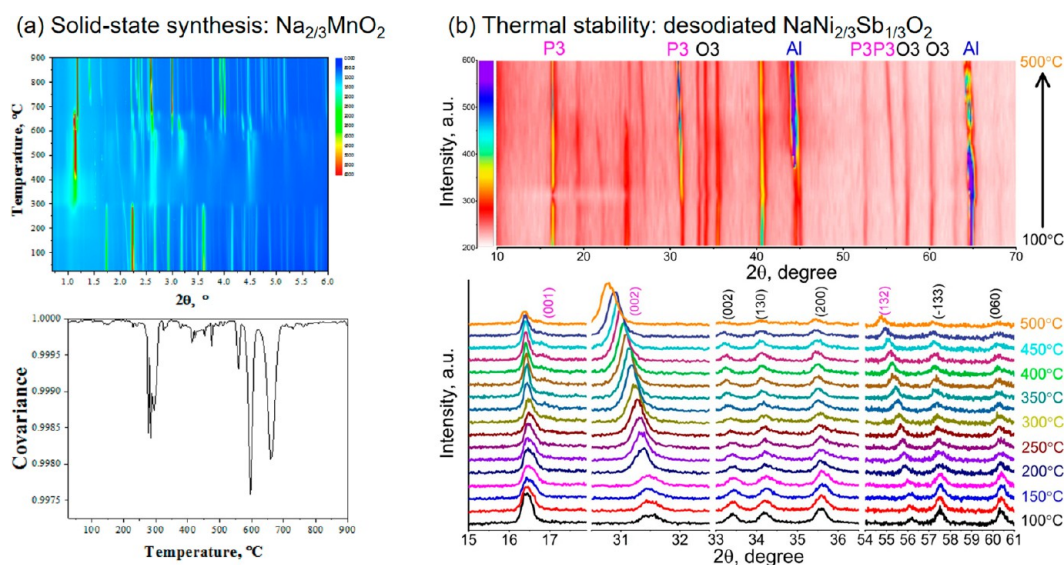
Figure 11. In situ/operando XRD investigation during materials synthesis and for thermal stability of electrode materials. (a) Contour plot of in situ XRD patterns collected during the solid-state synthesis and corresponding covariance analysis. Reprinted with permission from ref 139. Copyright 2017 Elsevier. (b) Contour plots of high-temperature in situ XRD patterns of charged state \text{NaNi}_{2/3}\text{Sb}_{1/3}\text{O}_2 electrode and corresponding selected diffraction patterns. Reprinted with permission from ref 140. Copyright 2017 Elsevier.
