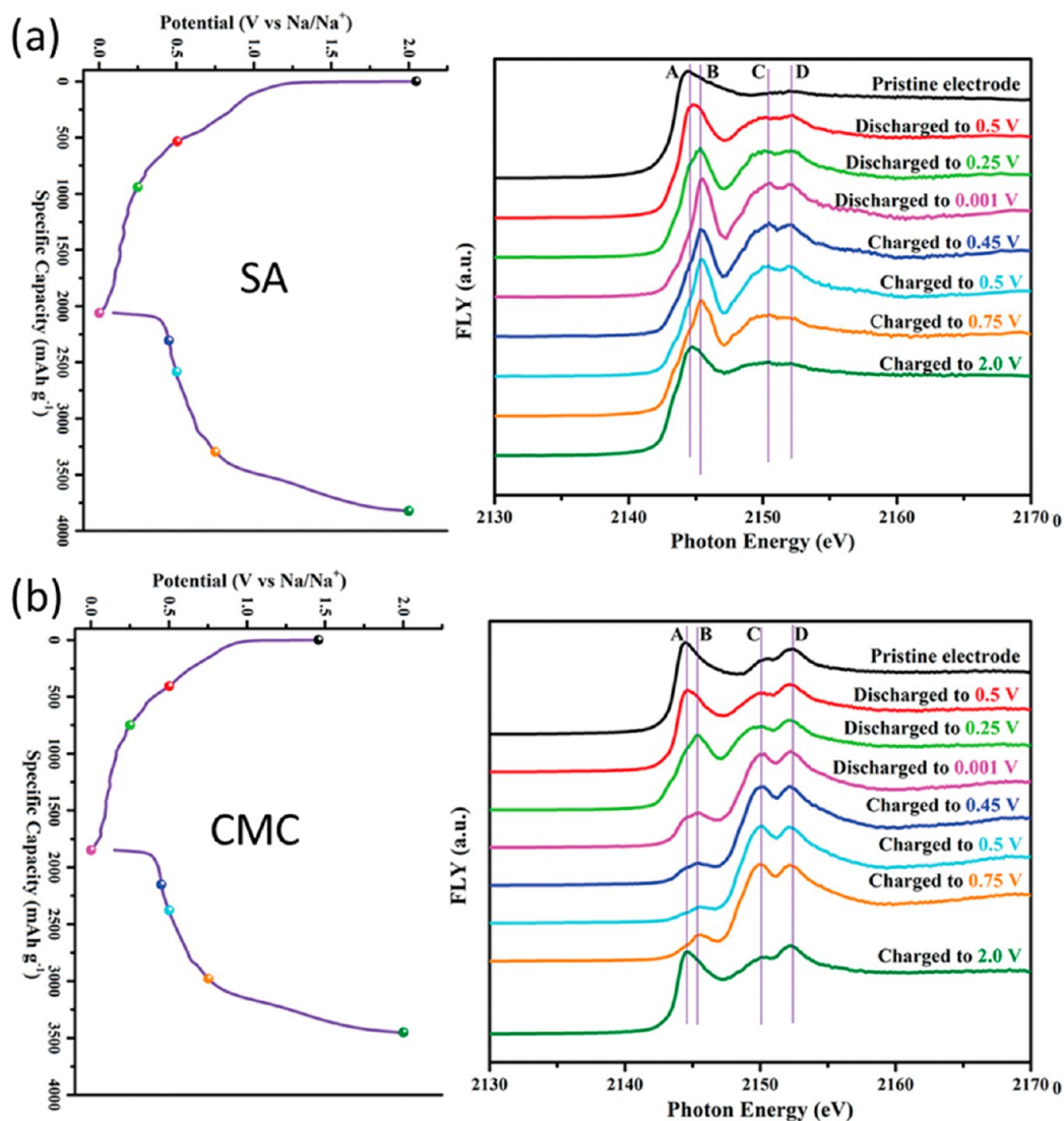
Figure 17. P K-edge of (a) sodium alginate-SA and (b) sodium carboxymethyl cellulose-CMC binders in electrodes at different charged/discharged states (left). Total fluorescence yield mode is applied. Reprinted with permission from ref 200. Copyright 2020 Wiley.
