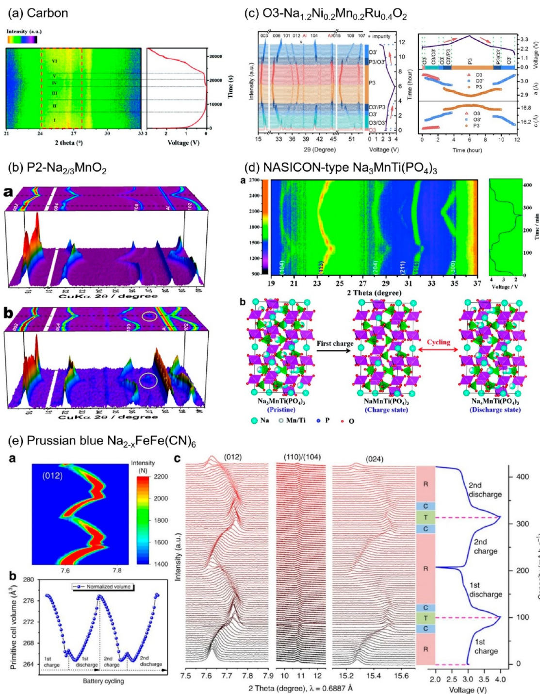
Figure 9. In situ /operando XRD investigations in intercalation-type electrode materials. (a) In situ XRD mapping of hard carbon anode during the first cycle at 200 mA g -1 at room temperature. Adapted permission from ref 97. Copyright 2017 Wiley. (b) Operando XRD of P2-Na 2/3 MnO 2 (top panel) and P2-Na 2/3 [Mn 0.8 Co 0.2 ]O 2 (bottom panel). Reprinted with permission from ref 111. Copyright 2019 American Chemical Society. (c) In situ XRD of Na 1.2 Ni 0.2 Mn 0.2 Ru 0.4 O 2 (left panel) and the corresponding lattice parameters evolutions (right panel). Adapted with permission from ref 120. Copyright 2018 Elsevier. (d) In situ XRD of the Na 3 MnTi(PO 4 ) 3 cathode cycled at 50 mA g -1 and schematic illustration showing Na + intercalating from/into Na 3 MnTi(PO 4 ) 3 cathode upon electrochemical processes. Adapted with permission from ref 122. Copyright 2019 Wiley. (e) 2D contour map of (012) reflection plan of Na 2-x FeFe(CN) 6 (top-left panel), and normalized volume during cycling obtained from in situ SXRD patterns (bottom-left panel), as well as (012), (110)/(104), and (024) reflection planes of in situ SXRD patterns (right panel). Reprinted with permission from ref 123. Copyright 2020 Springer Nature.
