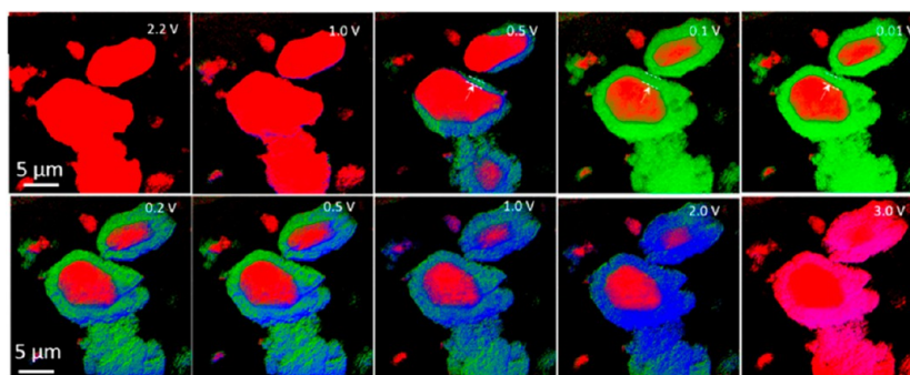
Figure 21. Reconstructed 2D chemical mapping images of CuO intercalated with sodium ions from in situ TXM. Reprinted with permission from ref 223. Copyright 2019 American Chemical Society.
