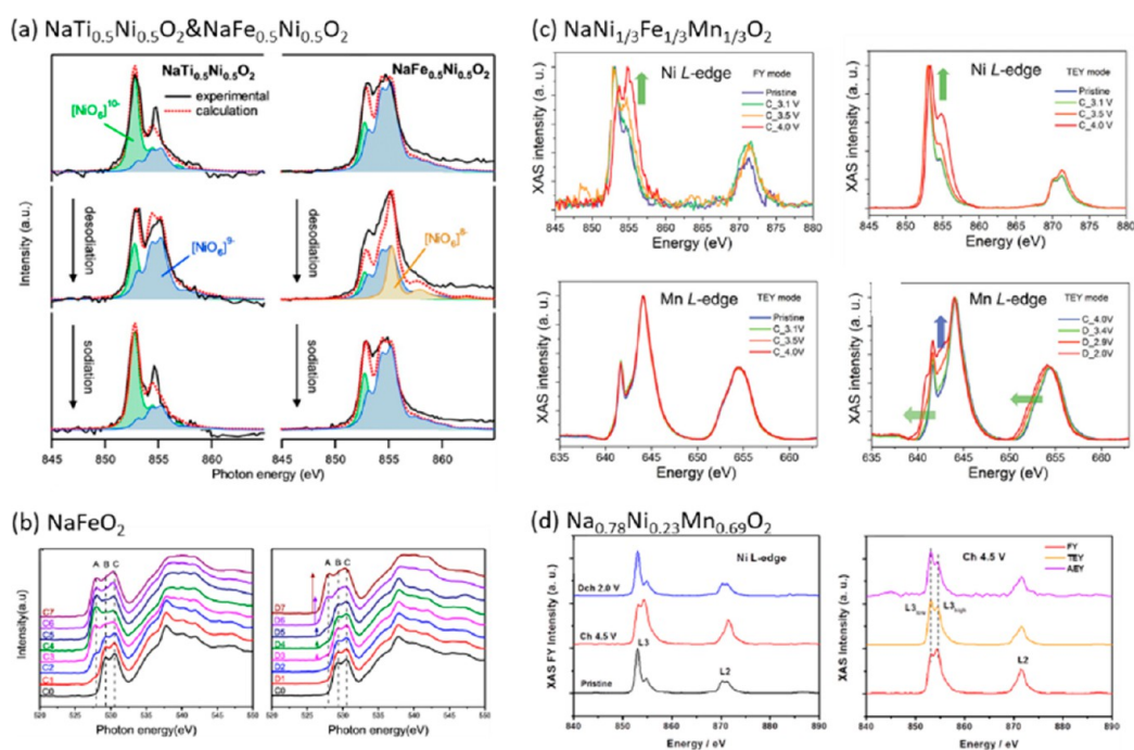
Figure 16. (a) Ni L-edge of \text{NaTi}_{0.5}\text{Ni}_{0.5}\text{O}_2 and \text{NaFe}_{0.5}\text{Ni}_{0.5}\text{O}_2 at different charged/discharged states in PFY mode. Linear combination was applied based on calculated patterns. Reprinted with permission from ref 175. Copyright 2016 American Chemical Society. (b) O K-edge \text{O}_3\text{-NaFeO}_2 at different charged/discharged states in TFY mode. C0-C7 means charging from 2.5 to 4.5 V continuously. D7-D1 is the reverse process. Adapted with permission from ref 159. (c) Mn and Ni L-edge of \text{NaNi}_{1/3}\text{Fe}_{1/3}\text{Mn}_{1/3}\text{O}_2 at different charged (C)/discharged (D) states. Ni was performed in total electron yield and fluorescence yield mode while Mn was under total electron yield mode. Reprinted with permission from ref 189. Copyright 2018 Wiley. (d) L-edge of Ni for \text{Na}_{0.78}\text{Ni}_{0.23}\text{Mn}_{0.69}\text{O}_2 . Adapted with permission from ref 195.
