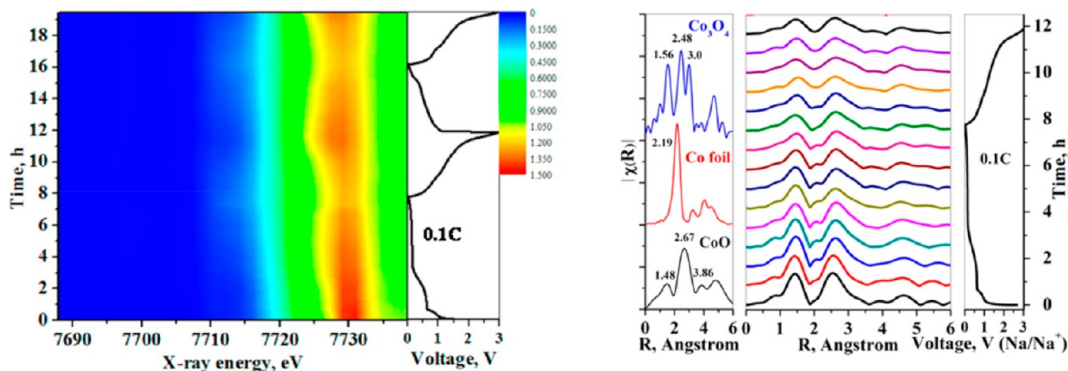
Figure 15. Operando XANES spectra and corresponding EXAFS analysis along with discharge/charge profiles of porous cobalt oxide electrode. Reprinted with permission from ref 167.
