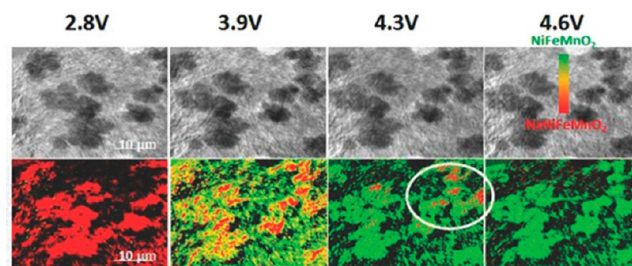
Figure 19. Reconstructed images of \text{NaNi}_{1/3}\text{Fe}_{1/3}\text{Mn}_{1/3}\text{O}_2 cathode at different states of charge derived from operando TXM. Reprinted with permission from ref 219. Copyright 2016 Wiley.
