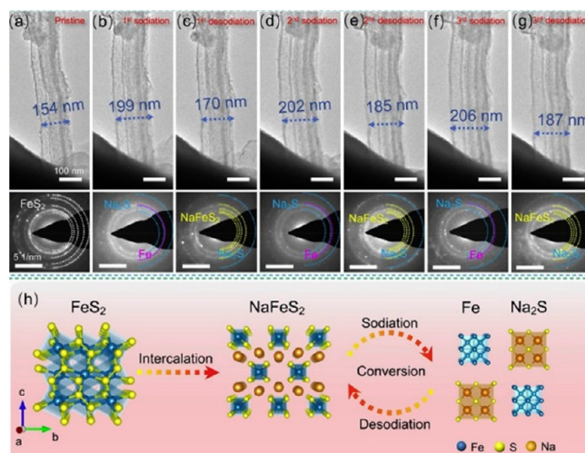
Figure 7. Intercalation–conversion reaction: FeS 2 . Reprinted with permission from ref 76. Copyright 2019 Elsevier.
