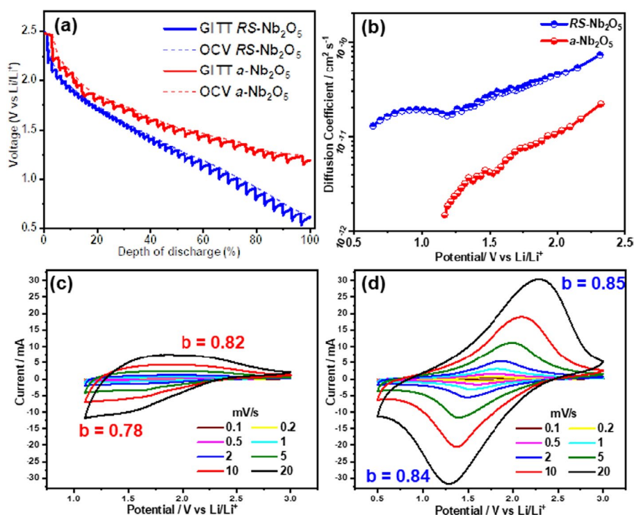
Extended Data Fig. 1 | Characterization of lithium ion diffusivity and charge storage of RS-Nb 2 O 5 and a -Nb 2 O 5 sample. a , GITT measurements of the RS- and a -Nb 2 O 5 electrodes. b , The logarithmic plot of Li ion diffusivity as a function of voltage by GITT measurements. Overall, RS-Nb 2 O 5 exhibited an order of magnitude higher Li ion diffusivity compared to a -Nb 2 O 5 within the potential window during lithiation. During the cathodic scan, both samples experienced a gradual decrease in diffusivity as more Li + occupied the vacant sites in the host material. It is worth noting that below 1.1 V, Li + diffusivity in RS-Nb 2 O 5 slightly increased, concurrent with the ongoing phase transformation upon cycling. Li + diffusivity in RS-Nb 2 O 5 is also higher than that of other polymorphs of Nb 2 O 5 electrodes. c and d , cyclic voltammograms of RS- and a -Nb 2 O 5 electrodes at varying scan rates. Insights in terms of diffusion and capacitive contribution to Li storage can be obtained by analyzing the peak current ( i ) dependence on scan rate ( ν ). For a redox reaction limited by semi-infinite diffusion, the peak current is proportional to the square root of the scan rate ( ν 1/2 ); while for a capacitive process it varies linearly with ν 44,45 . A b value can be obtained by analyzing the power law relationship between i and ν via i = a\nu^b , where a and b are adjustable parameters. It was found that the b values for RS-Nb 2 O 5 and a -Nb 2 O 5 sample were -0.85 and -0.80, respectively. The results suggest both electrodes have mixed contribution from diffusion and capacitive process with RS-Nb 2 O 5 electrode having a slightly higher capacitive contribution indicative of a faster kinetic in RS-Nb 2 O 5 .
