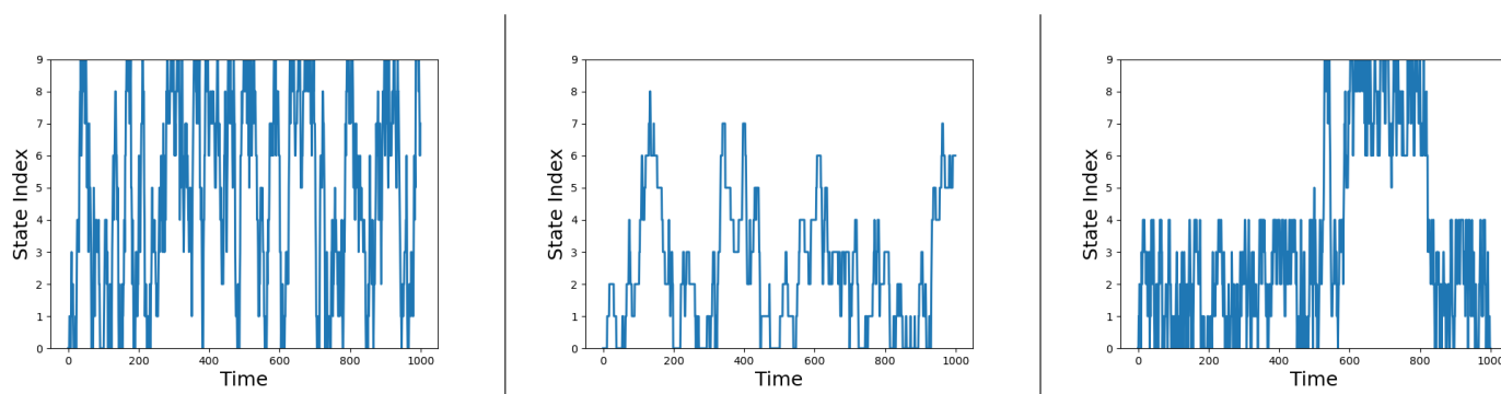
Figure 7. Three examples of the state index trajectory in an expanded ensemble simulation in one dimension. On the left, the simulation travels from top to bottom state multiple times, suggesting good mixing of states on this timescale. In the center, jumps between states are occurring slowly, and the simulation is not spanning the entire state range, suggesting the spacing between states may need to be decreased (i.e. overlap between states increased), or weights may need to be improved. On the right, we have a bottleneck in the middle of the states, preventing the overall simulation from mixing easily through the entire range of states. Although states and 0–4 and 5–9 can mix readily, the overall traversal of state space is slow, and the overlap and weights of that transition should be examined to improve sampling. For similar replica exchange cases, see Figure 5.
